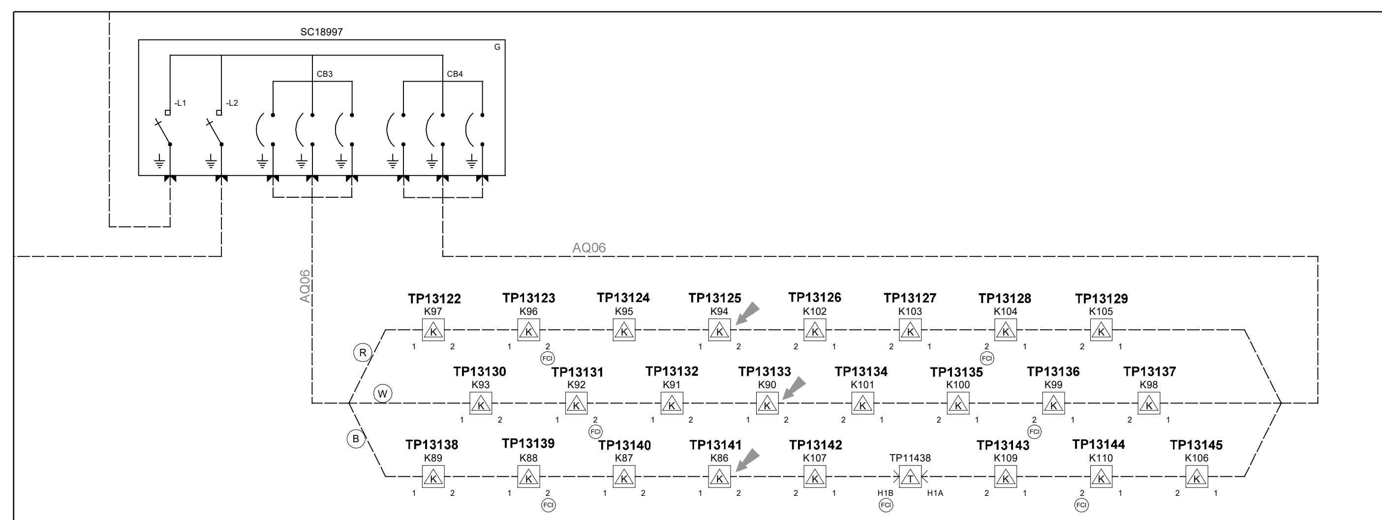
EXISTING / PROPOSED SINGLE LINE DIAGRAM N.T.S.
