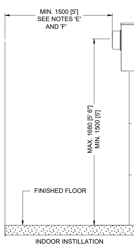
FIG. 1 REVENUE METERING EQUIPMENT
