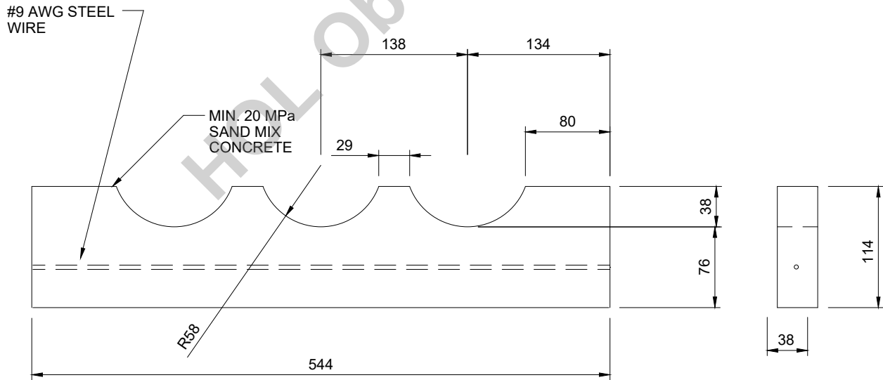
BASE SPACER
