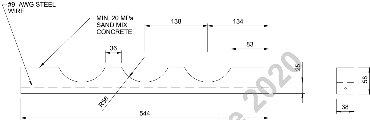
INTERMEDIATE SPACER
