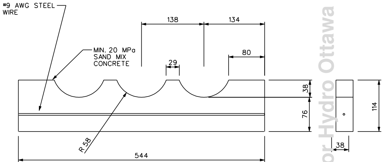
BASE SPACER
