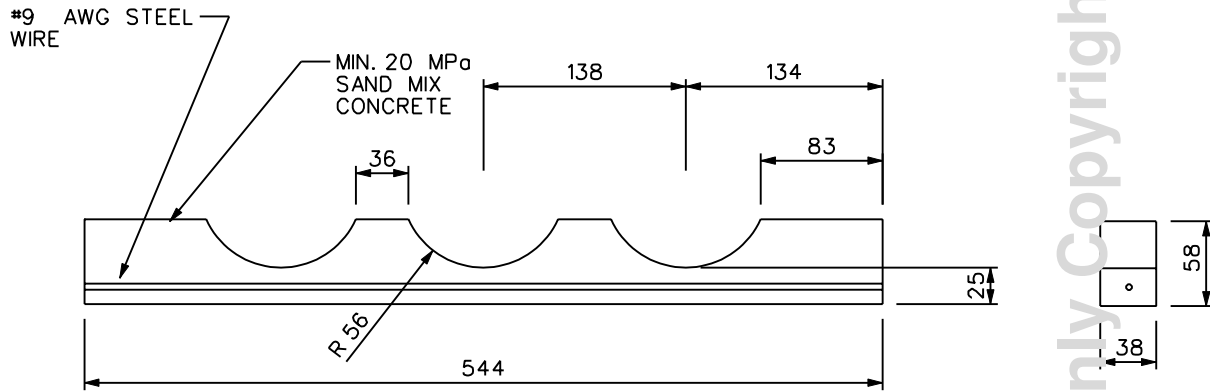
INTERMEDIATE SPACER
