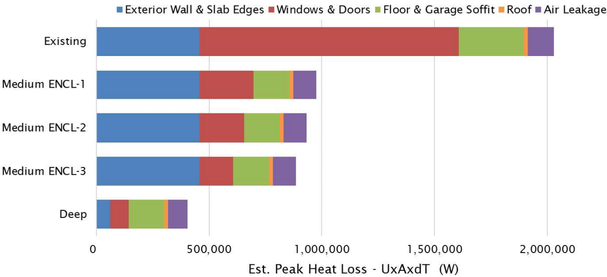
ESTIMATED HEAT LOSS THROUGH THE ENVELOPE FOR EACH RETROFIT PATH
