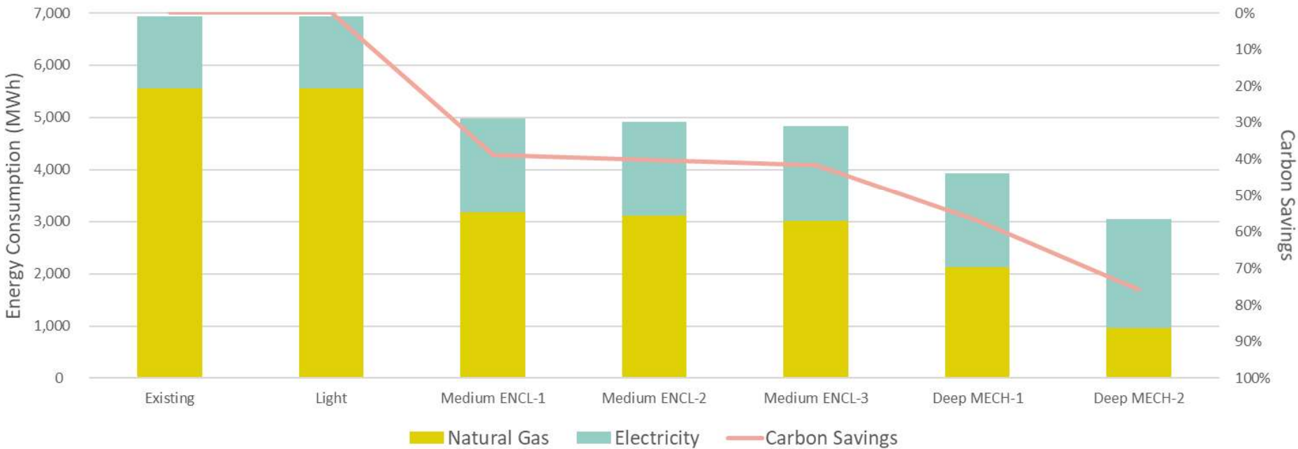
NATURAL GAS, ELECTRICITY USE AND CARBON SAVINGS FOR EACH RETROFIT PATH
