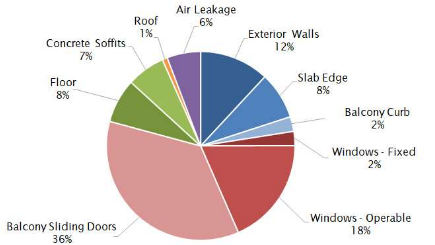
COMPONENTS OF STEADY STATE HEAT LOSS THROUGH THE EXISTING BUILDING ENCLOSURE (ASHRAE DESIGN DAY CONDITIONS)
